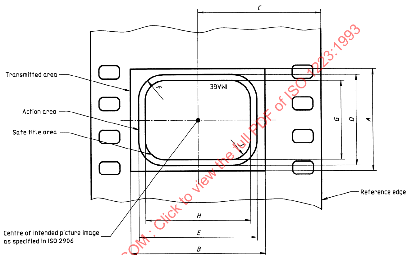
Figure 1 — Image area on 35 mm motion-picture film for television
