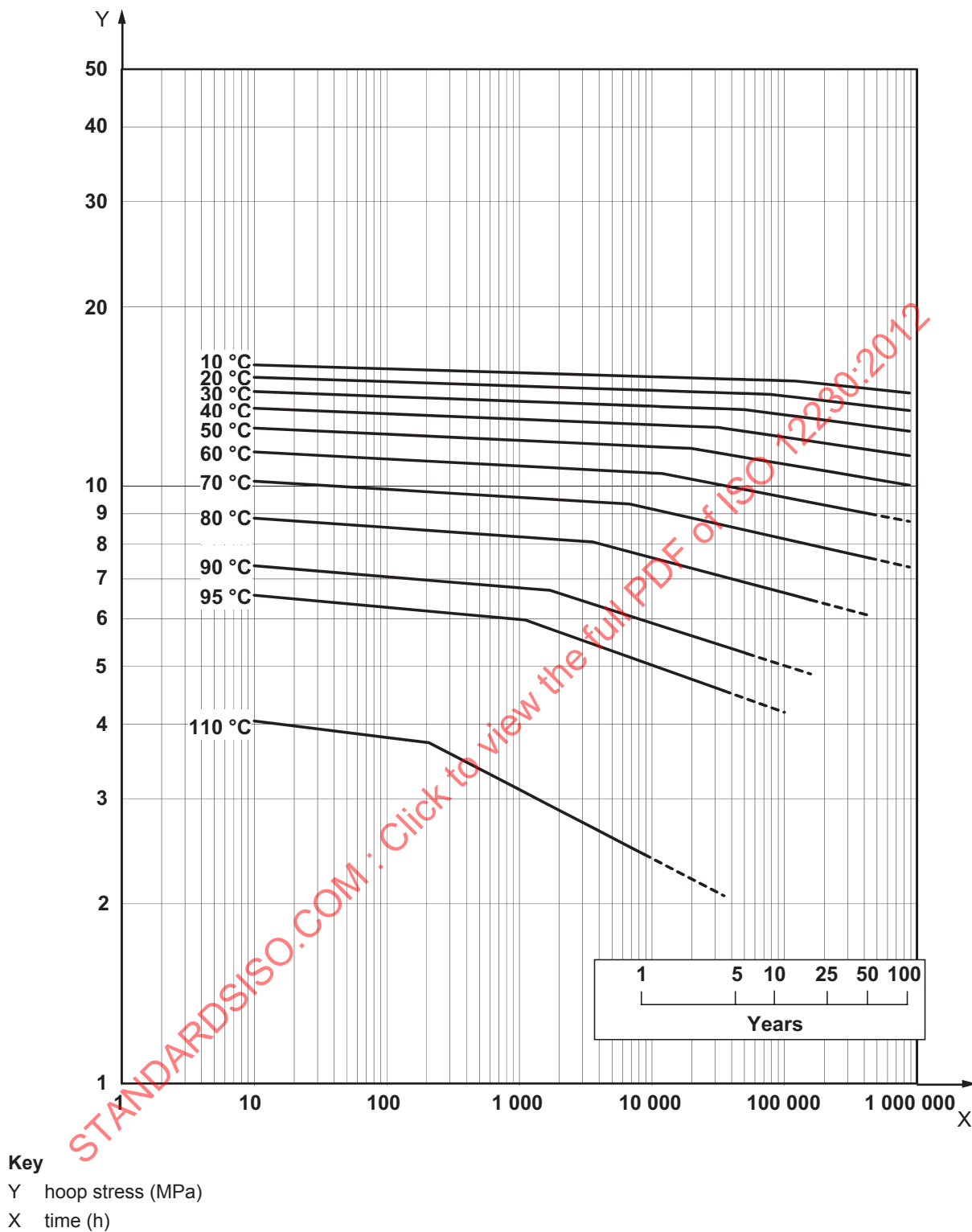
Figure 1 — Expected strength of polybutene homopolymer (PB-H) pipes
