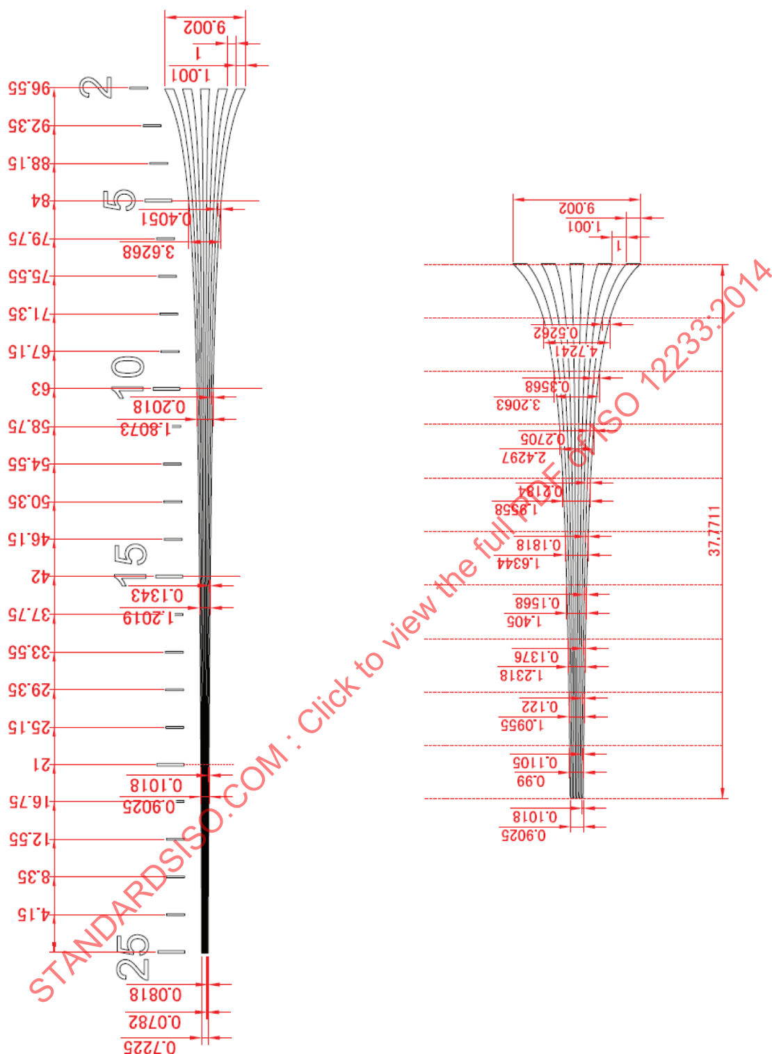
Figure A.5 — Detail drawing for five-line hyperbolic wedge pattern
