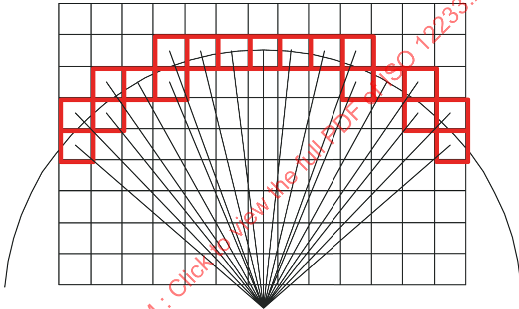
Figure F.3 — Location of pixels along a specific radius
