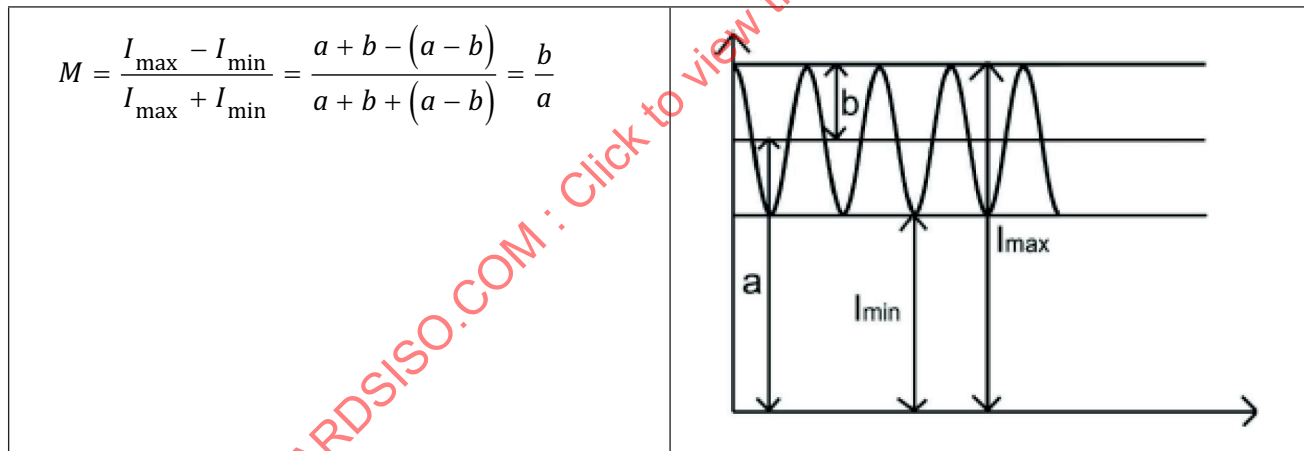
Figure F.5 — Calculation of the contrast of the sine curve
