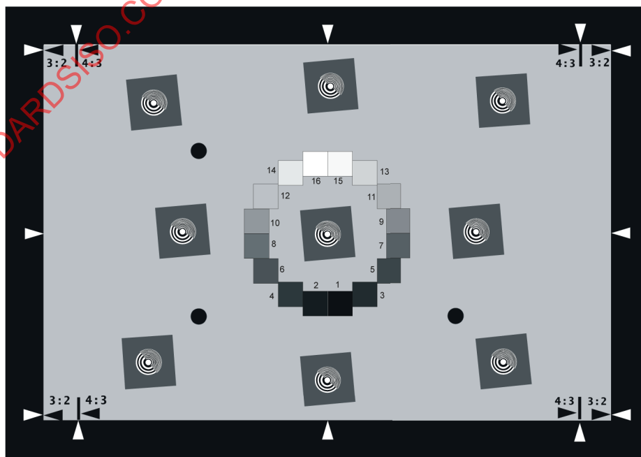
Figure 4 — Low contrast e-SFR test chart
