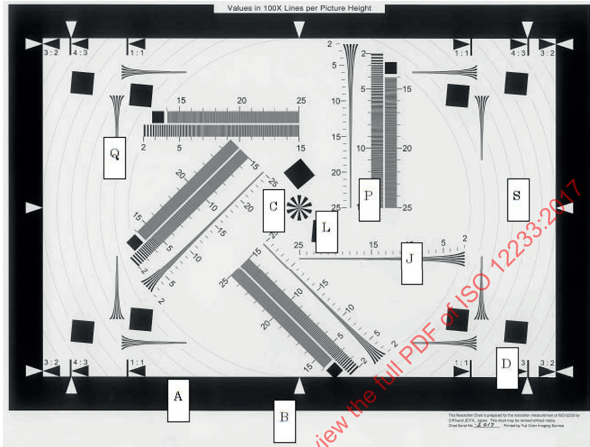
Figure A.1 — Characteristics of the visual resolution test chart
