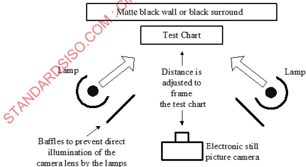
Figure 1 — Test chart illumination method
