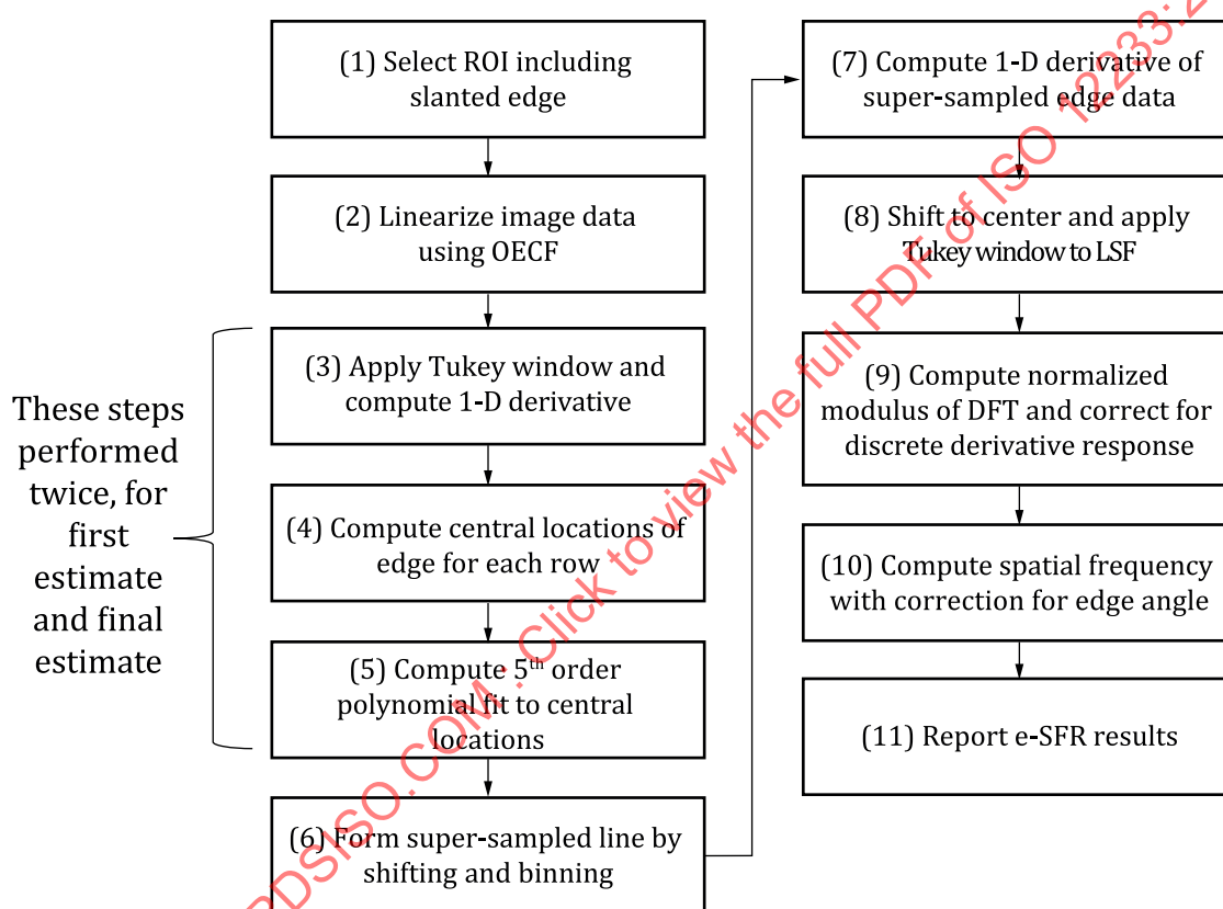
Figure D.1 — Flowchart of e-SFR measurement algorithm
