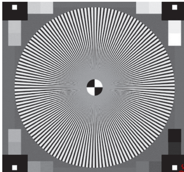
Figure 6 — Sine-based SFR test chart
