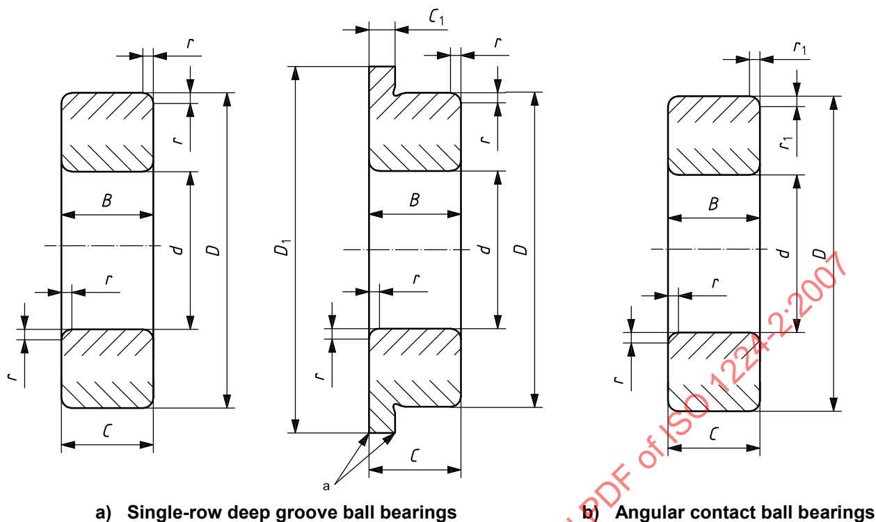
Figure 1 — Instrument precision bearing
