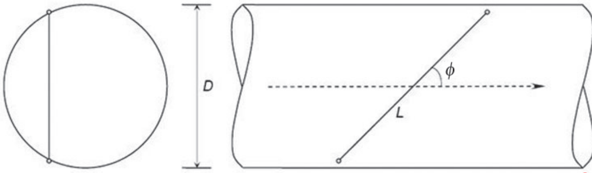
Figure 1 — Measurement principle
