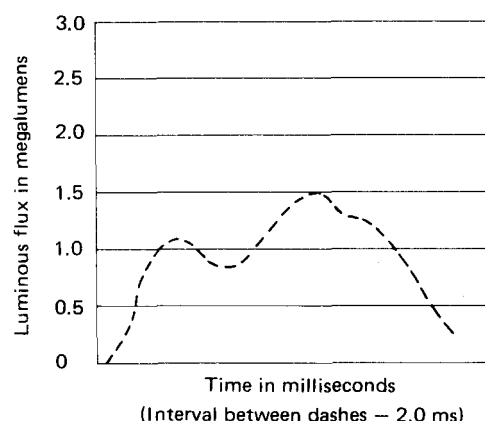
FIGURE 2 – Luminous flux versus time curve
