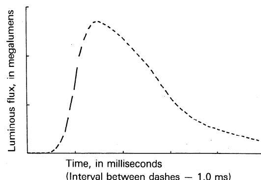
Figure 2 — Luminous flux versus time curve
