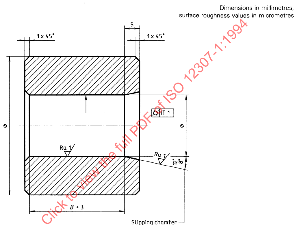
Figure 7 — Ring gauge
