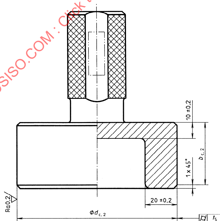
Figure 6 — Setting plug, for example with blind hole, for d_{c,2} > 80 mm
