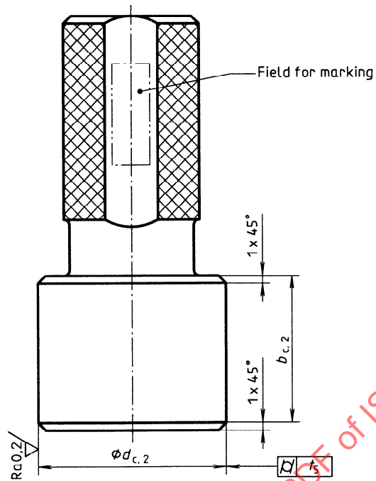
Figure 5 — Setting plug, solid, for d_{c,2} \leq 80 mm
