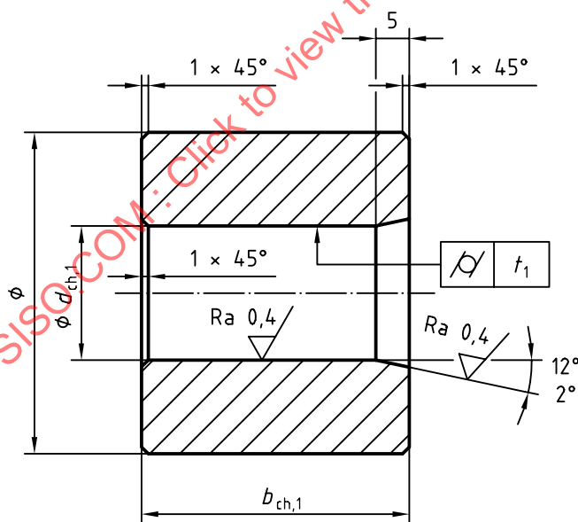
Figure 1 — Ring gauge
