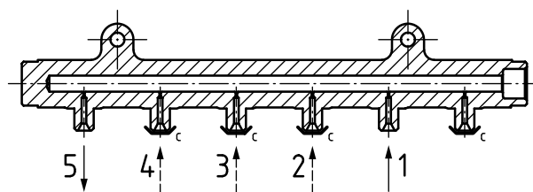
Figure B.2 — Step 1 of the test procedure
