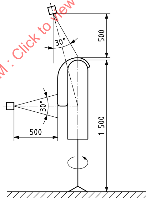
Figure 11 — Test apparatus for automatic inflation devices
