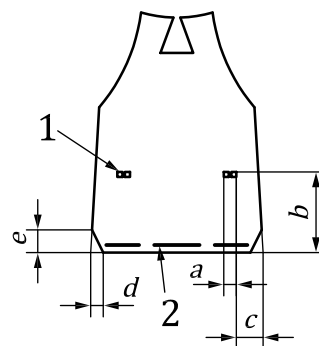
Figure B.13 — Attachments to inside cover (dimensions on pattern, before sewing)
