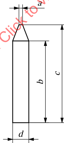
Figure B.4 — Centre gusset
