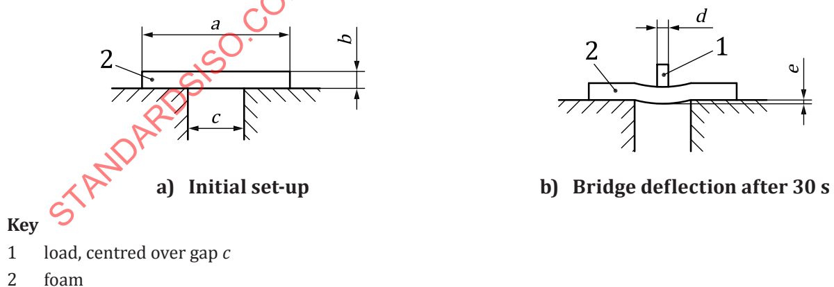
Figure B.1 — Foam bridge deflection test
