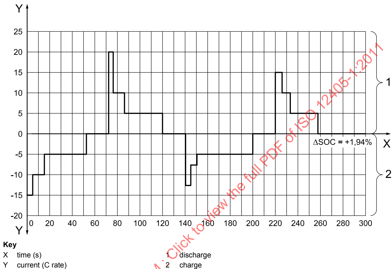
Figure 8 — Current profile for cycle life test — Charge-rich profile
