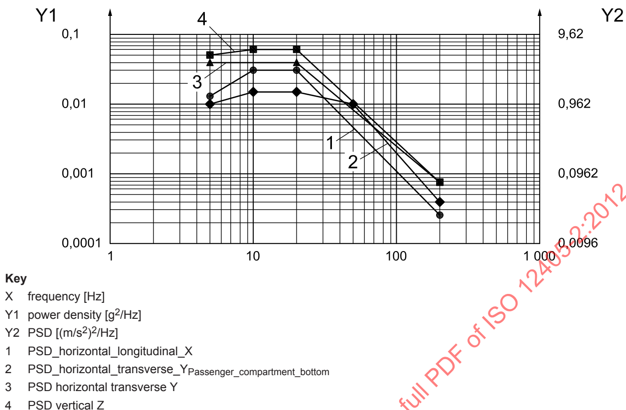
Figure 12 — PSD spectra for sprung masses (masses mounted on vehicle body)
