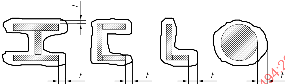
Figure 3 — Ice accretion model for glaze
