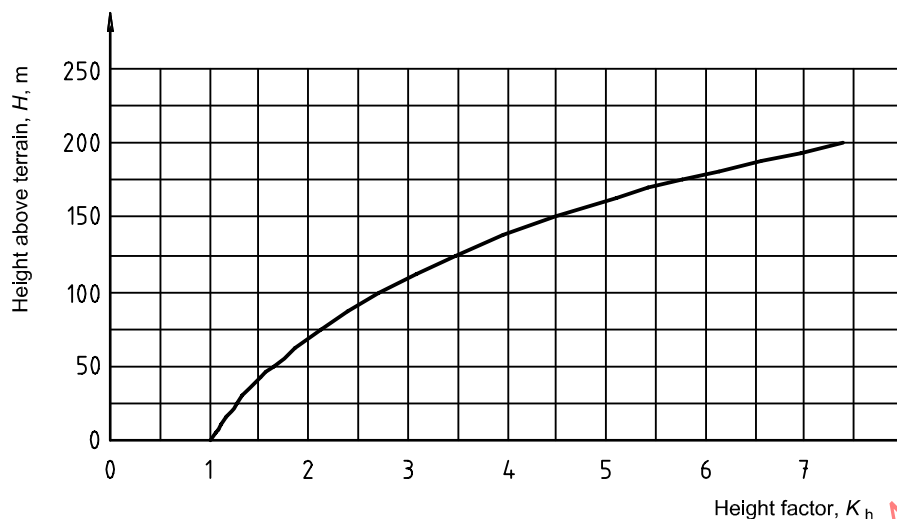
Figure 2 — Typical variation of ice masses with the height above terrain
