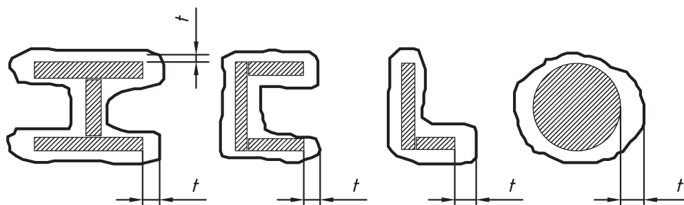
Figure 3 — Ice accretion model for glaze
