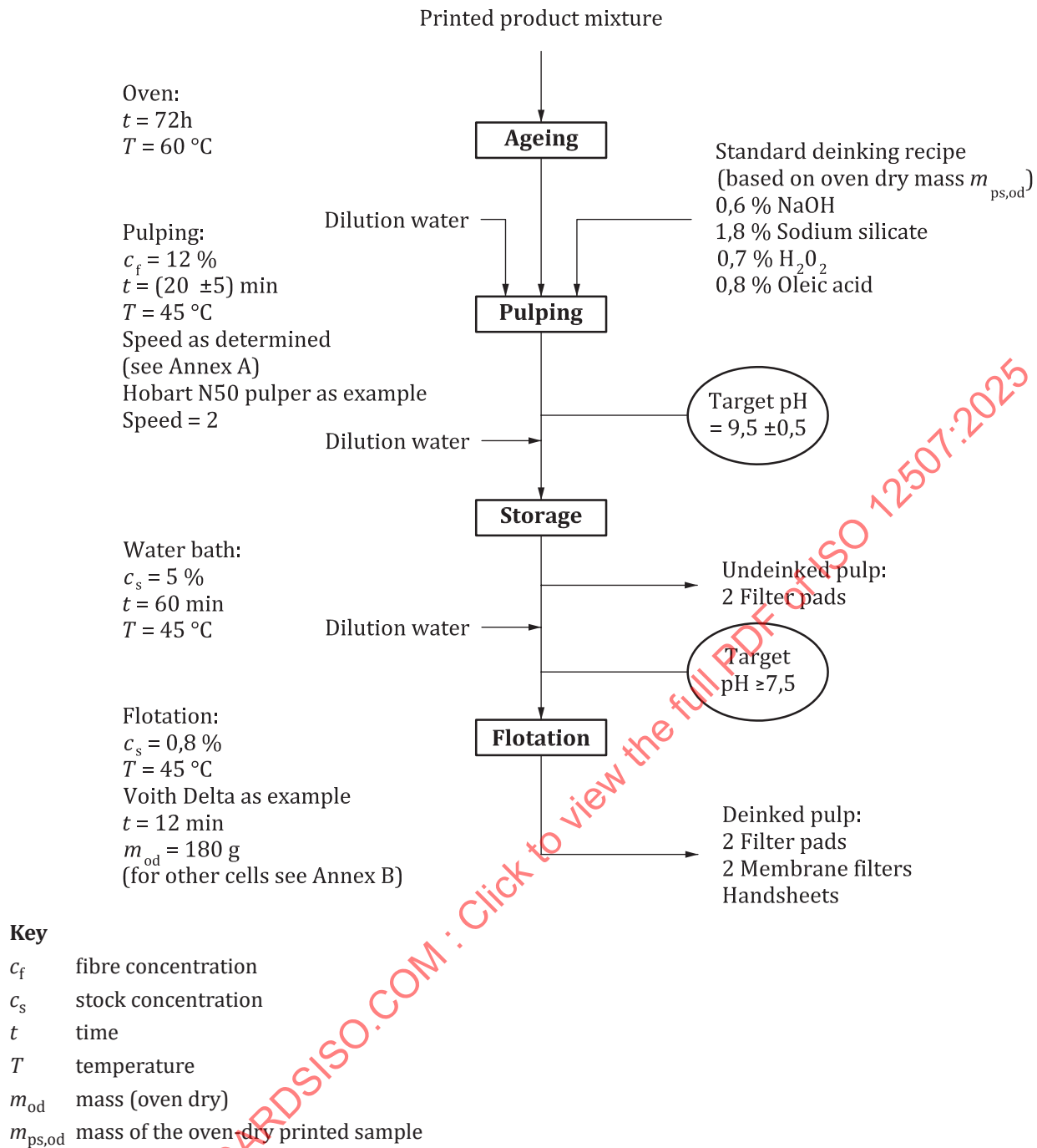
Figure 1 — Procedure for testing deinkability with standard deinking recipe
