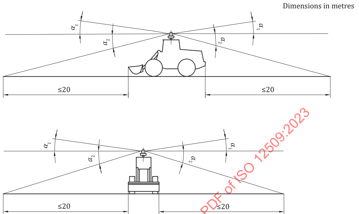
Figure C.12-1 — Special warning lamp
