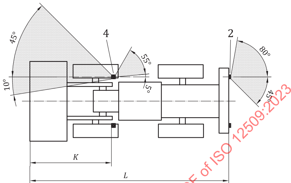
b) Arrangement B
