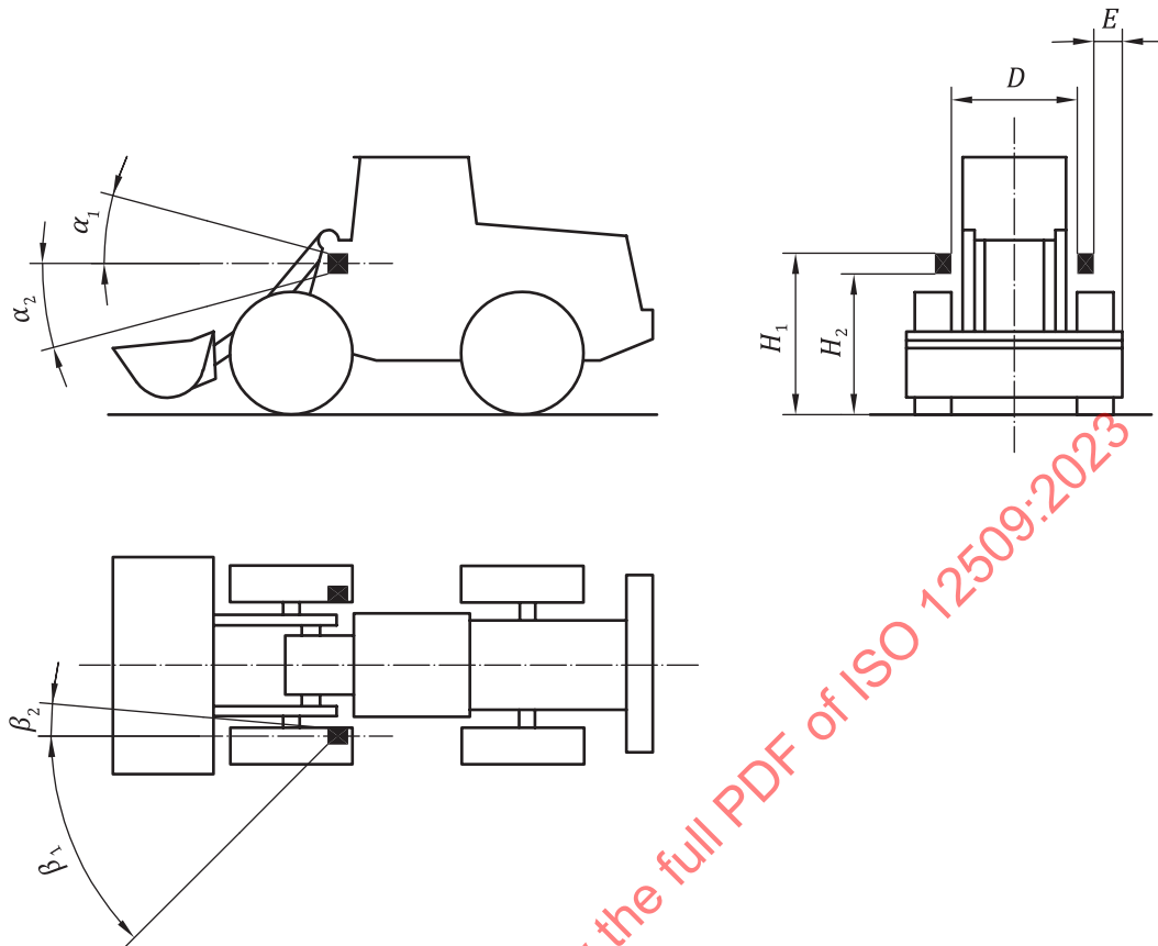
Figure C.2-1 — Upper beam headlight
