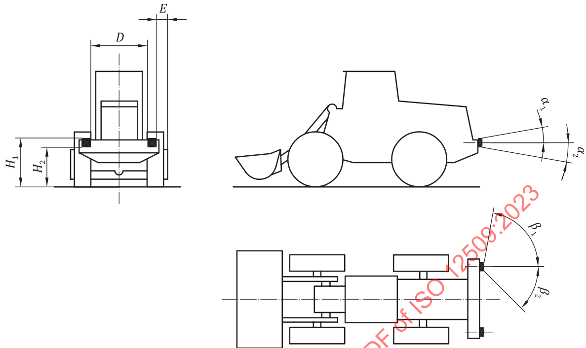
Figure C.10-1 — Rear position lamp
