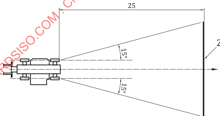
b) Rearward visibility zone of no white light from a lamp or white reflex reflector [see 4.1.6 b) ]
