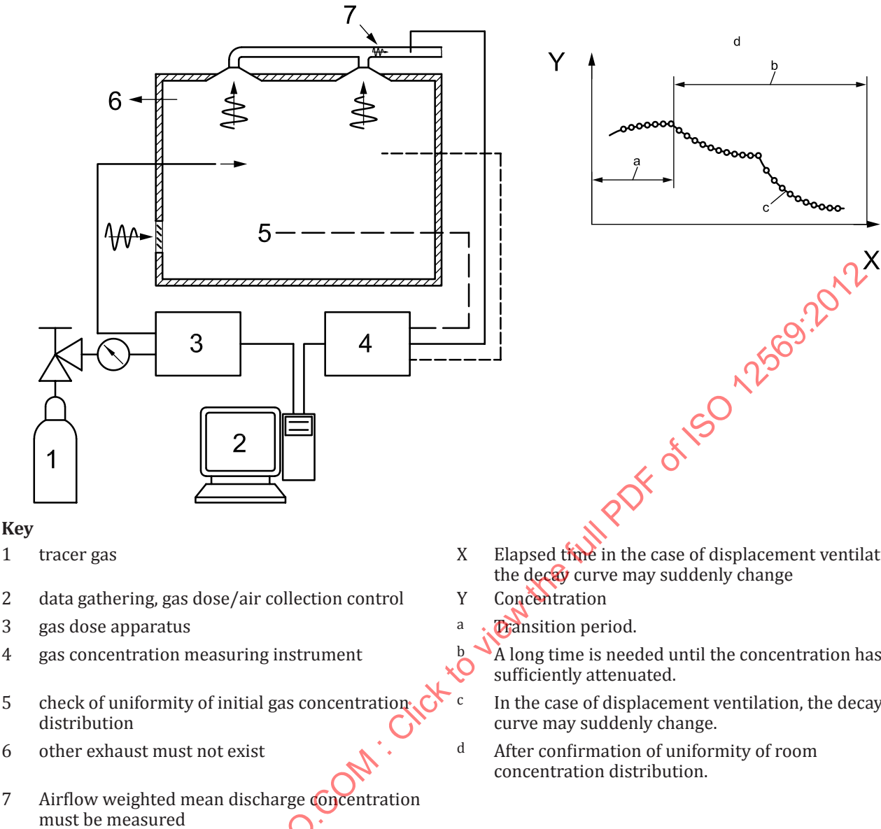
Figure 2 — Overview of step-down exhaust concentration method
