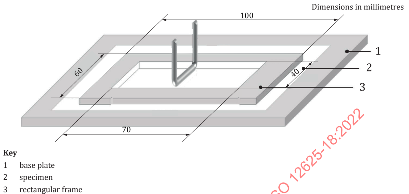
Figure 2 — Arrangement of the specimen holder
