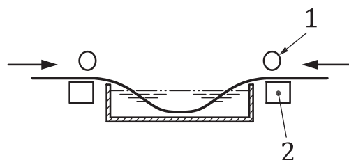
Figure 3 — The two clamps, the soaking device filled with water and the test piece inserted between the two clamps
