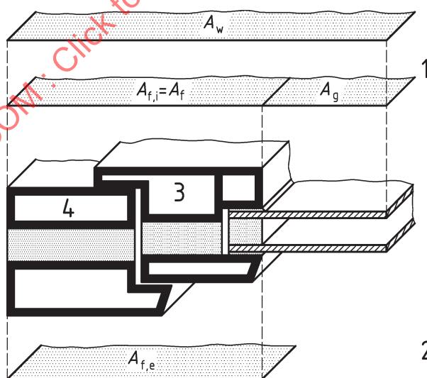
Figure 14 — Illustration of the various areas on frame-sash sections and glazing
