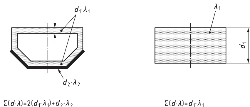
Figure B.1 — Definition of glazing unit spacer bars with improved thermal performance
