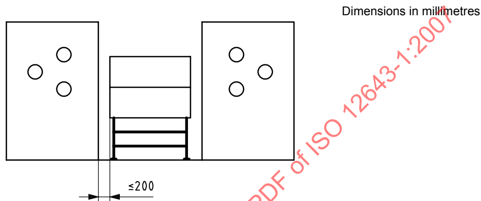
Figure 17 — Mobile platform
