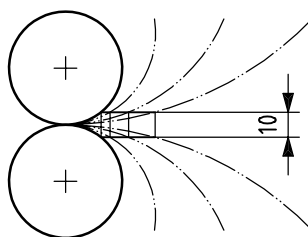
Figure 3 — Measuring safety distance at the in-running nips
