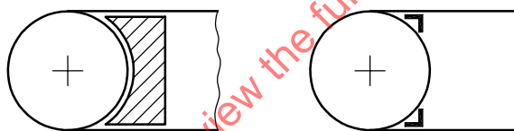
Figure 11 — Safeguarding of belt in-running nips on belt drives
