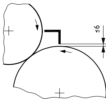
Figure 6 — Safeguarding an in-running nip by means of a fixed nip guard
