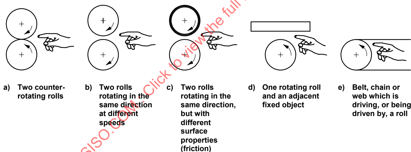
Figure 1 — In-running nips
