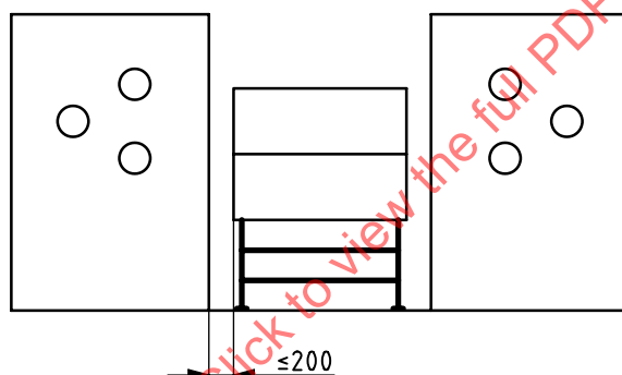
Figure 17 — Mobile platform
