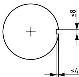
Figure 1 — Smooth roller/cylinder
