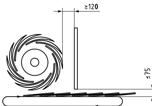
Figure 6 — Openings for folder guards
