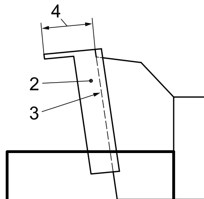
Figure 4 — Relationship between safety device and platen trip bar
