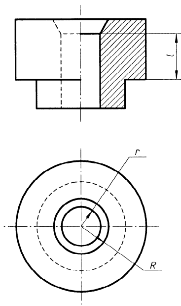
Figure 2 — Aperture ring
