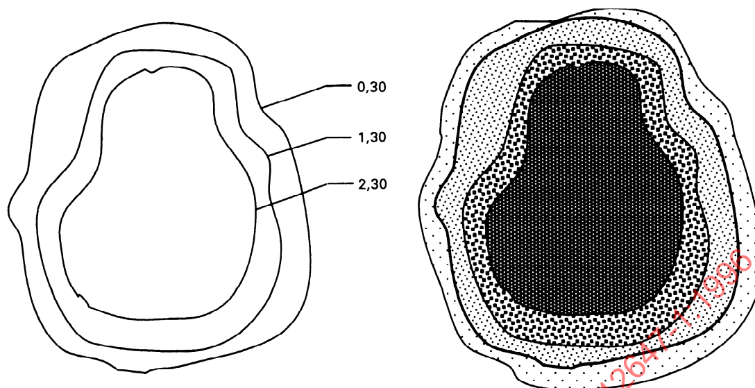
Figure B.2 — Example for the transmittance density contour lines of a soft half-tone dot on a colour separation film (left), microscopic image of the same dot (right)
