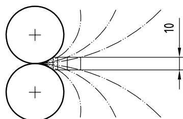
Figure 3 — Measuring safety distance at in-running nips
