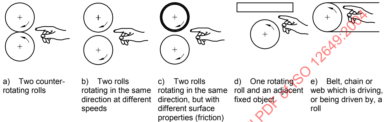
Figure 1 — In-running nips
