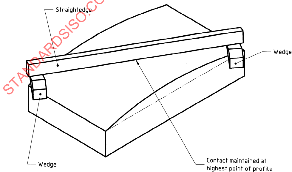
Figure 4 — Measurement of convex warpage
