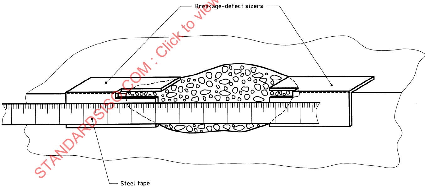
Figure 8 — Measurement of the length of an edge defect
