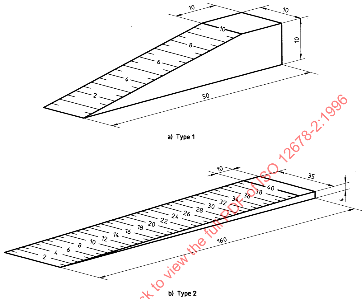
Figure 4 — Two types of measuring wedge
