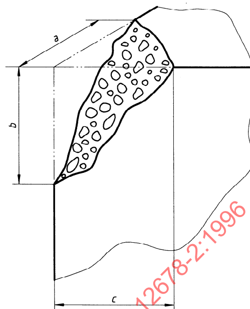
Figure 1 — Typical corner defect
