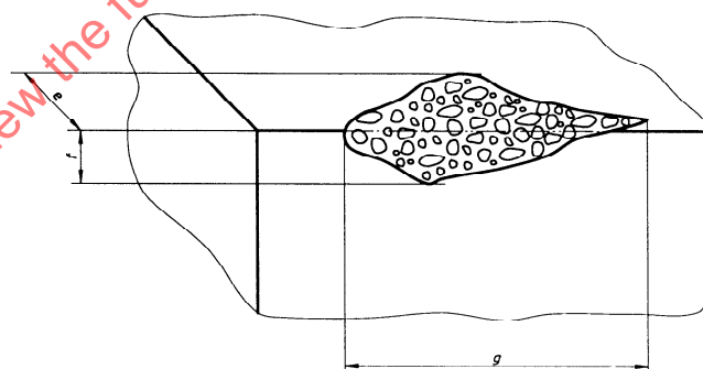
Figure 2 — Typical edge defect
