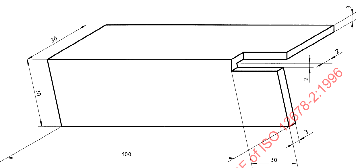
Figure 5 — Breakage-defect sizer
