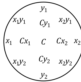
Figure B.3 — Test type A2/B2 circular thickness measurement pattern
