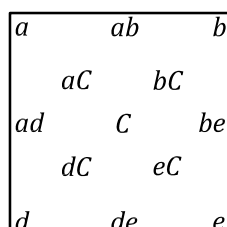
Figure B.2 — Test type A2/B2 thickness square measurement pattern
