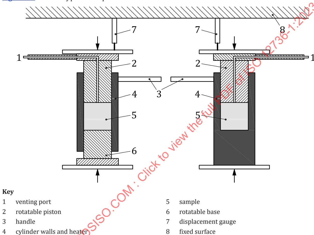
Figure C.5 — Typical set up for tri-axial tests
