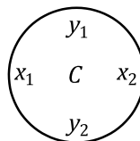
Figure B.1 — Test type A1/B1 thickness measurement pattern
