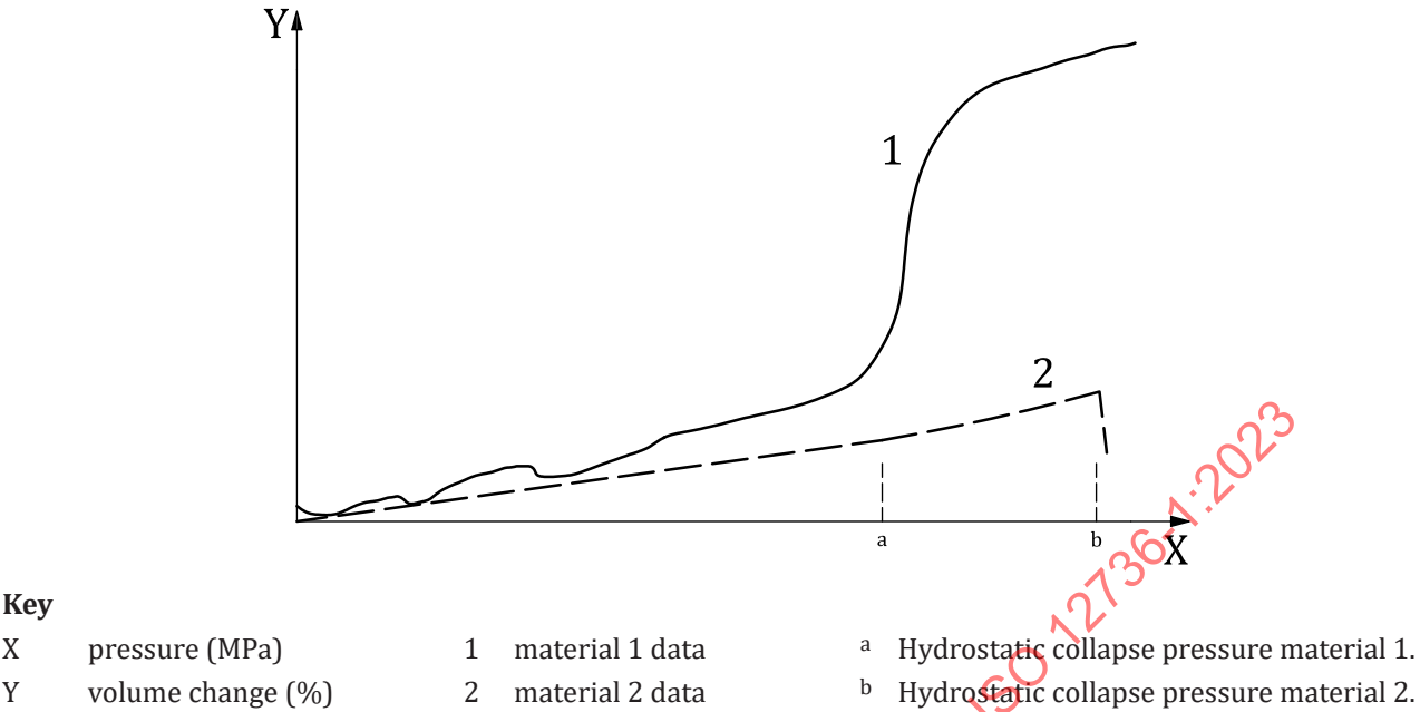
Figure C.3 — Typical chart of volume reduction as a function of pressure
