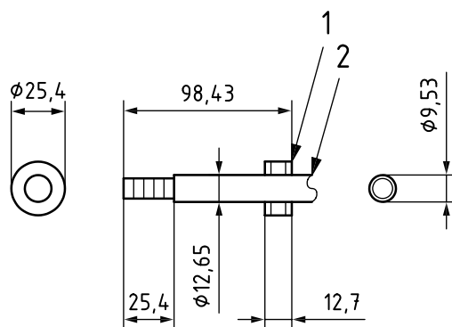
a) Cam shaft in medium-carbon tool steel
