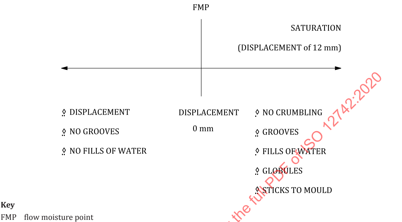
Figure 4 — Identification of the flow state
