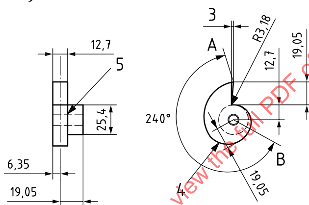
a) Cam shaft in medium-carbon tool steel
