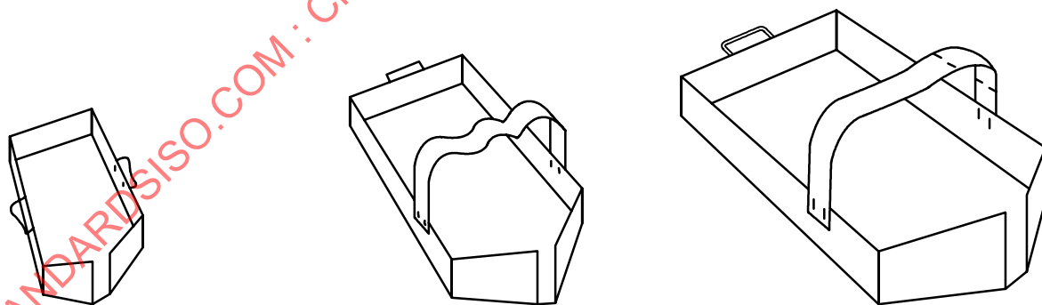
Figure 8 — Mixing trays
