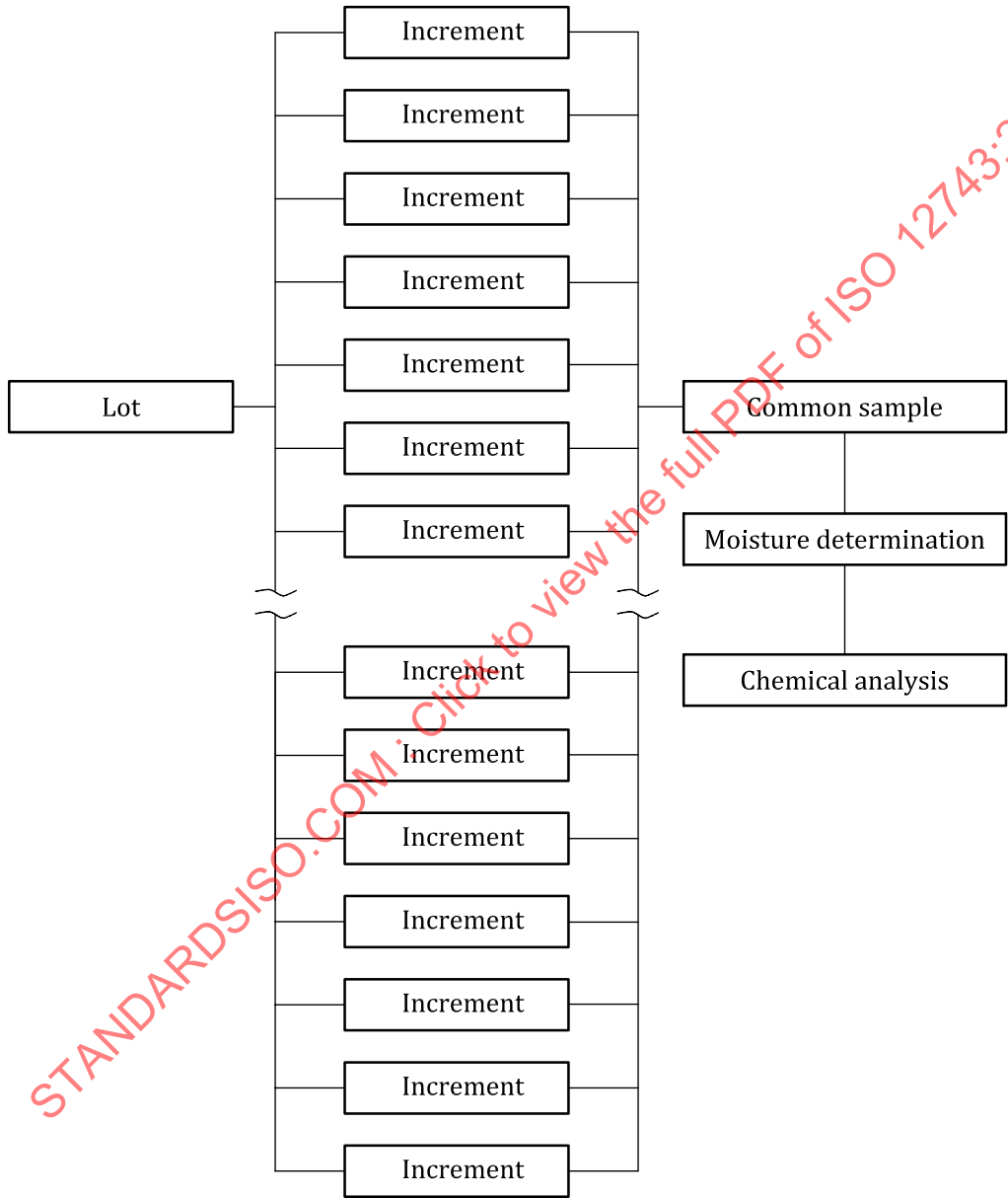
Figure 2 — Example of a sampling scheme in which a common sample is constituted for the lot for moisture determination and subsequent chemical analysis
