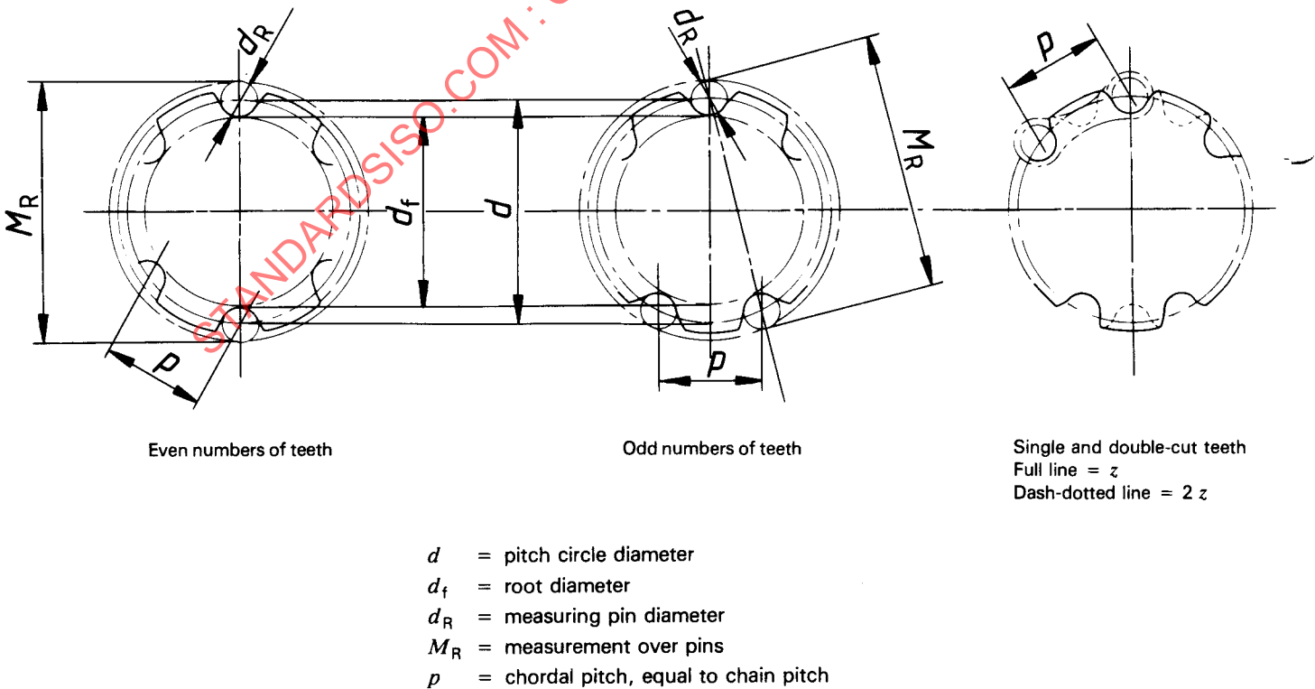
Figure 5 — Measuring pin size
