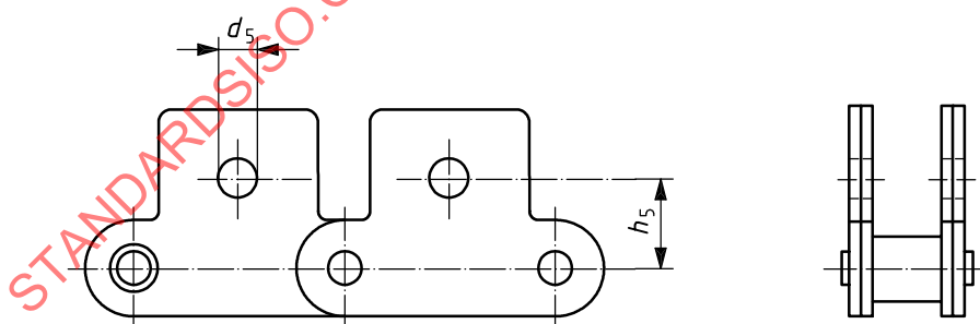
Figure 5 — K attachment plates
