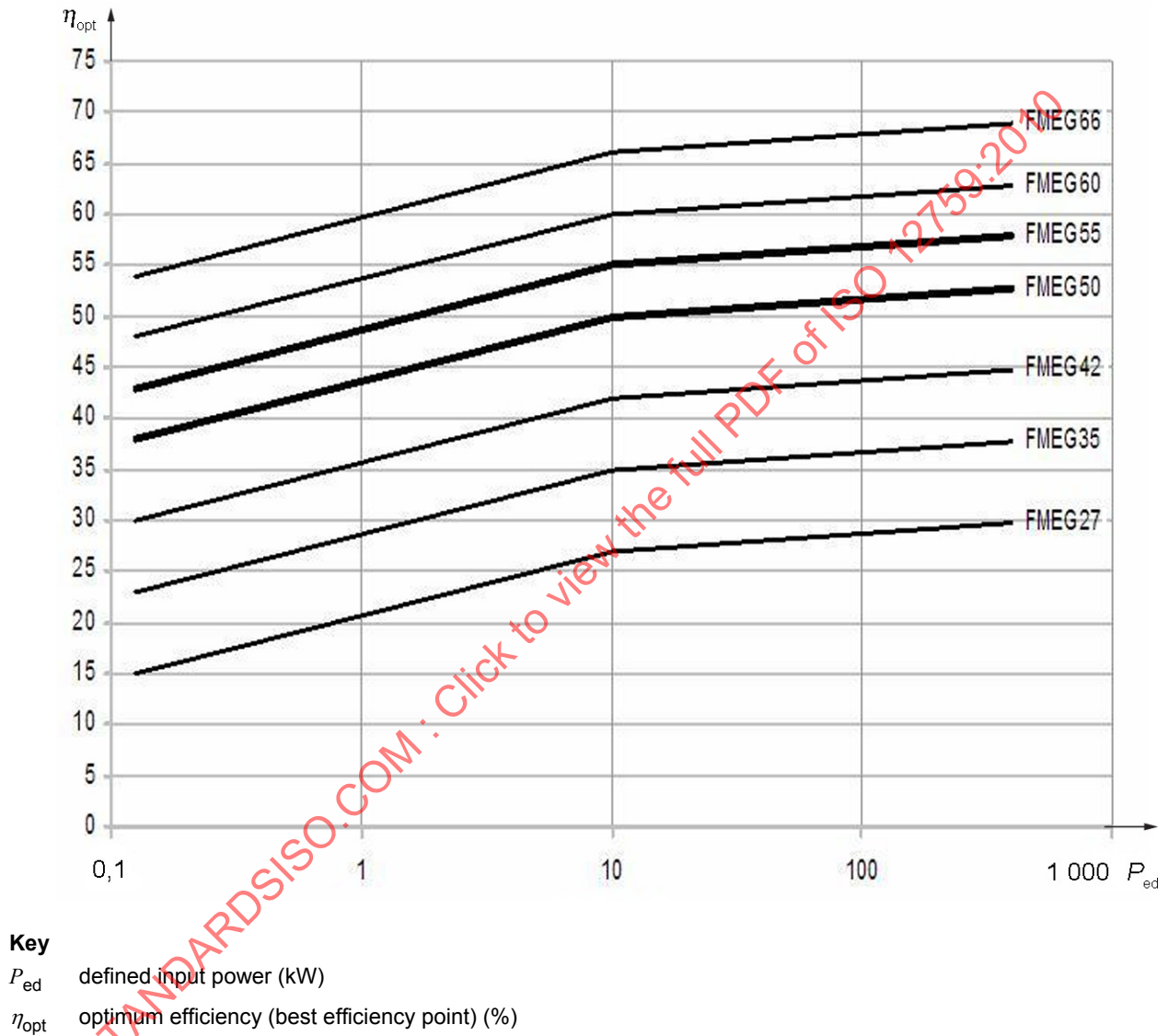
Figure 6 — Efficiency grades for axial, forward curved or radial-bladed centrifugal driven fans
