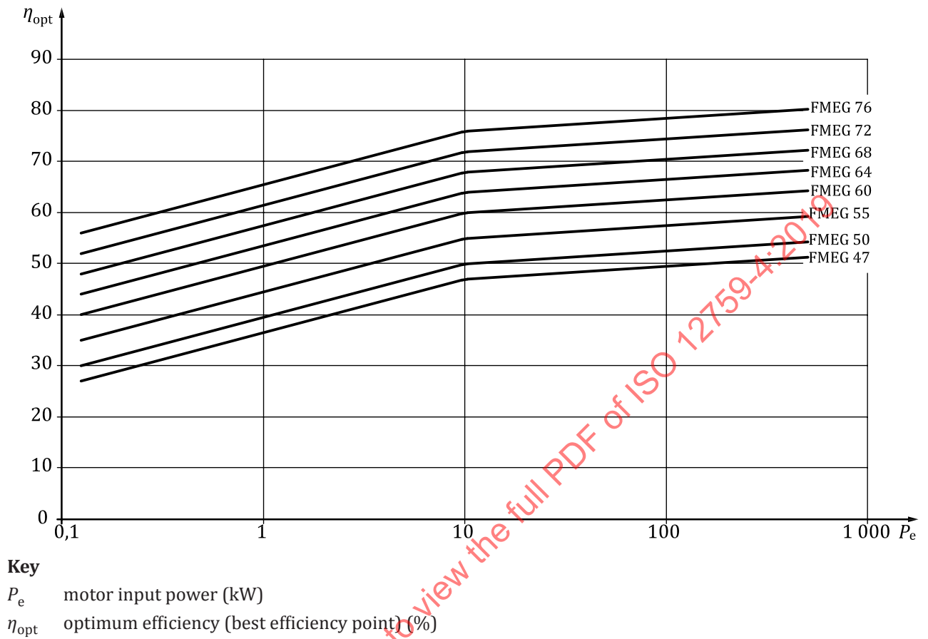
Figure 4 — Centrifugal backward bladed fan with and without housing driven fan efficiency grades
