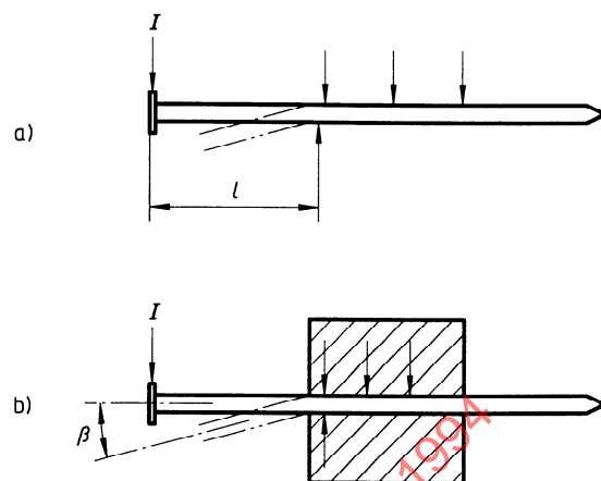
Figure 4 — Principle of the three-point impact method by impact load (impulse) I , showing angle of deformation \beta
