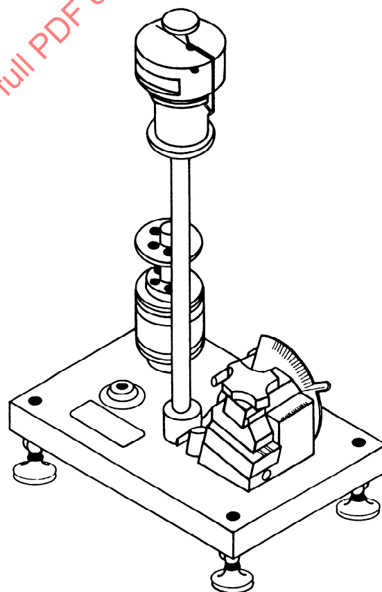
Figure 5 — Typical test apparatus — Three-point impact method
