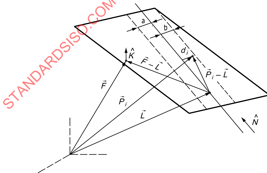
Figure A.1 — Straightness tolerance zone of a nominal integral feature
