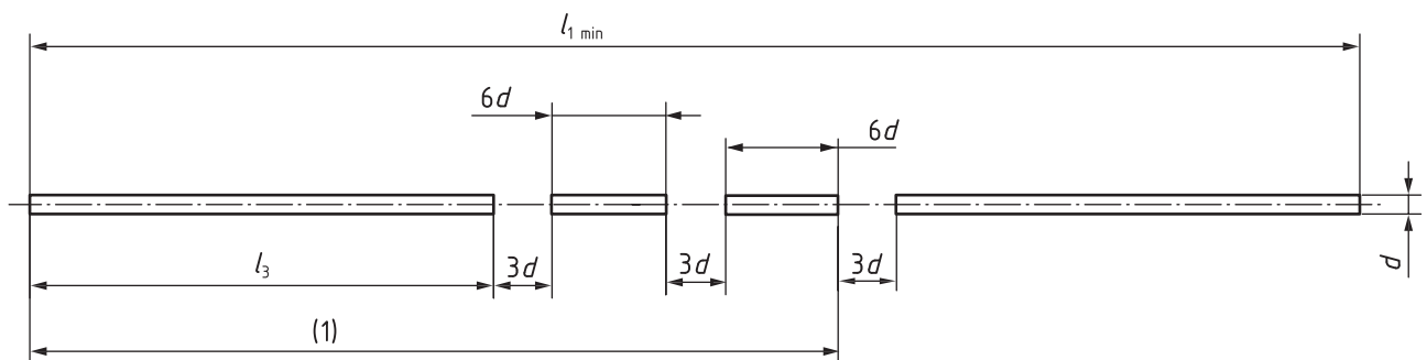
Figure A.14 — Configuration of line type no. 09 (long-dashed double-short-dashed line)
