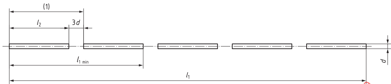
Figure A.4 — Configuration of line type no. 02 (dashed line)
