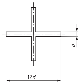
Figure 15 — Cross intersection
