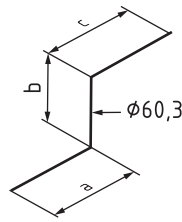
Figure 36 — Example of a reference line for dimension being omitted
