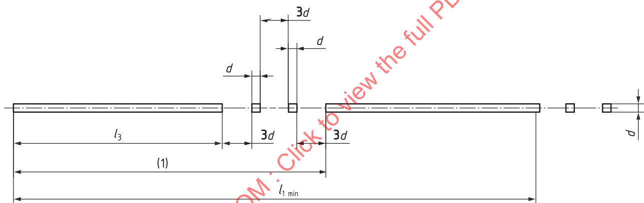
Figure A.8 — Configuration of line type no. 05 (long-dashed double-dotted line)
