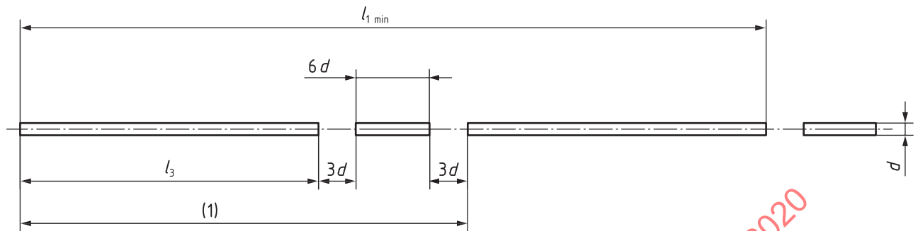
Figure A.13 — Configuration of line type no. 08 (long-dashed short-dashed line)
