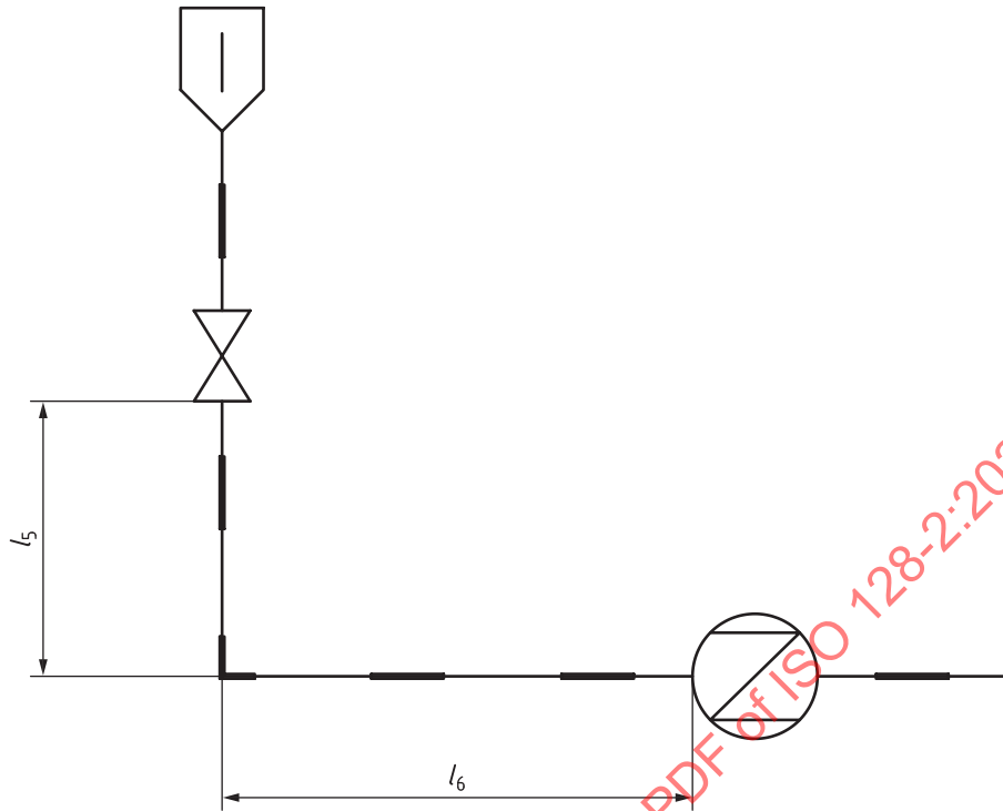
Figure A.16 — Example of two types of lines superimposed
