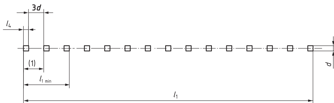
Figure A.11 — Configuration of line type no. 07 (dotted line)
