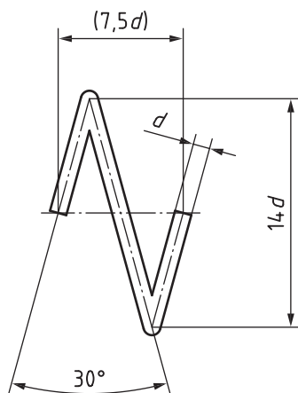
Figure A.17 — Configuration of line with zigzags
