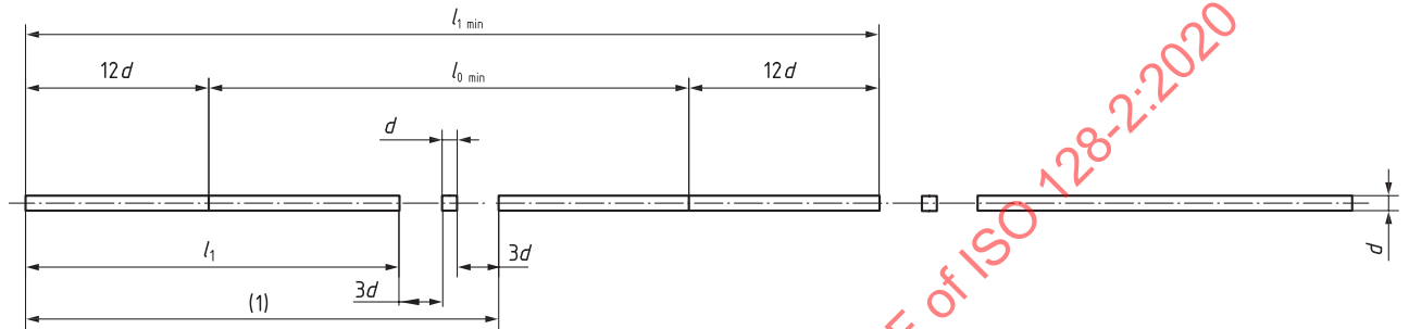
Figure A.6 — Configuration of line type no. 04 (long-dashed dotted line)
