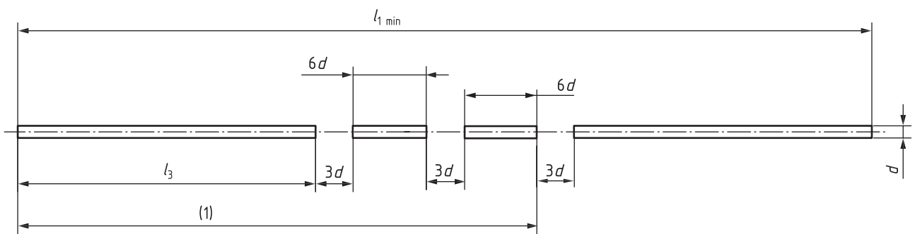
Figure A.14 — Configuration of line type no. 09 (long-dashed double-short-dashed line)
