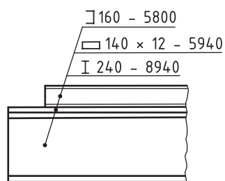
Figure 40 — Example of assembled parts of an object designated with one leader line
