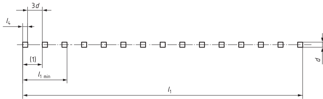
Figure A.11 — Configuration of line type no. 07 (dotted line)
