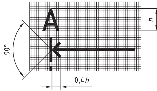
Figure A.4 — 90° cut and section arrow
