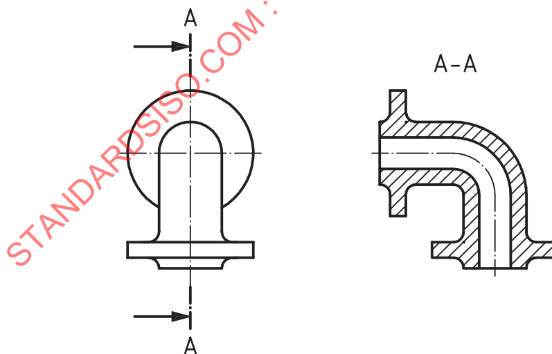
Figure D.1 — Section/cut in one plane
