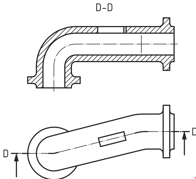
Figure D.4 — Section/cut in three contiguous planes
