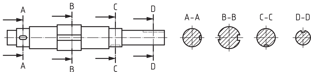
Figure D.8 — Successive sections/cuts — Example 1
