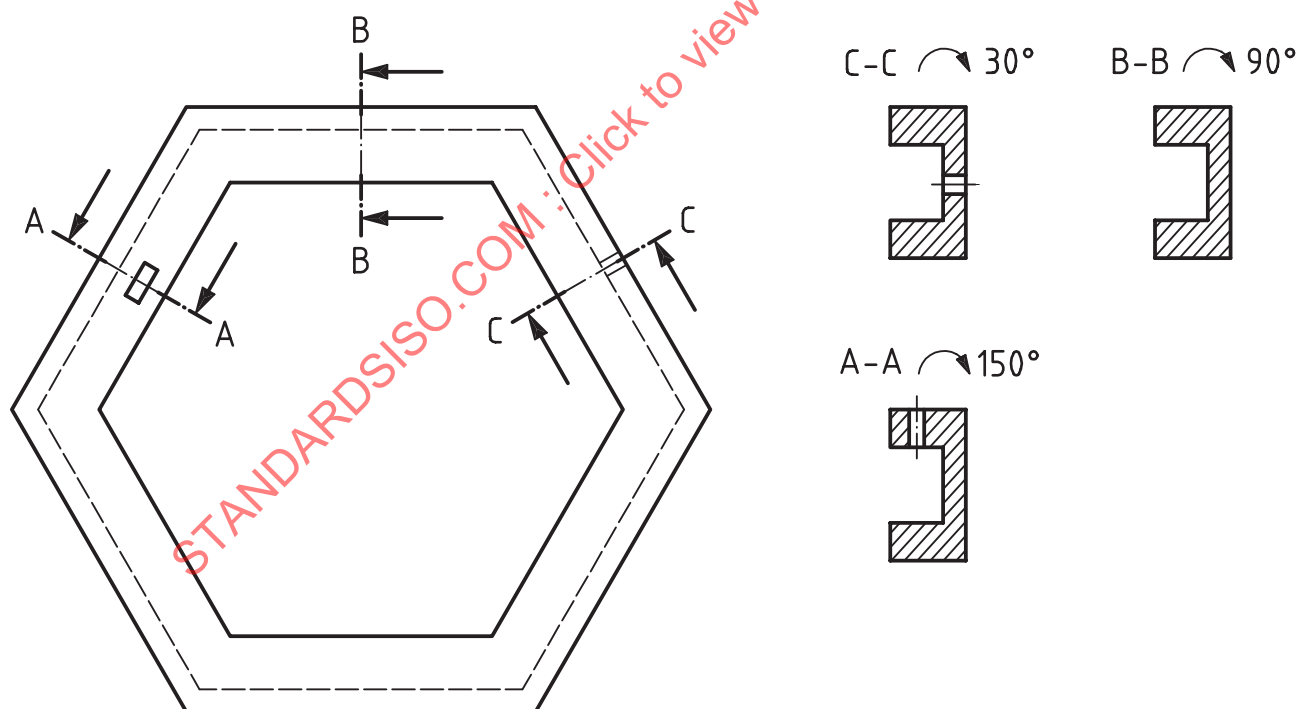
Figure D.10 — Successive sections — Example 3
