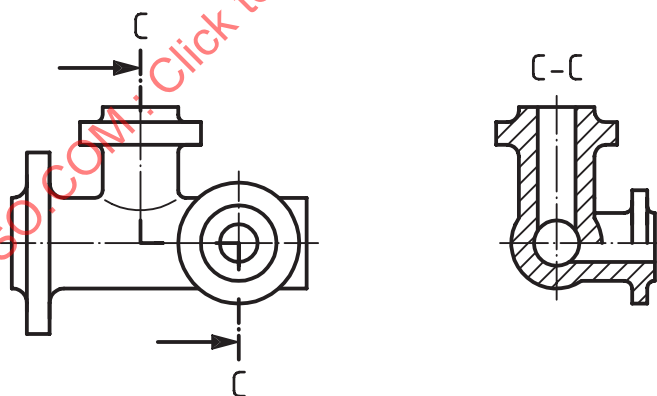
Figure D.3 — Section/cut in two parallel planes
