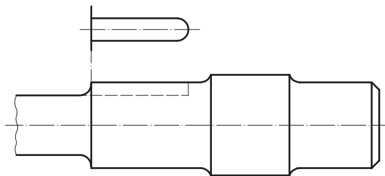
Figure C.4 — Local view of groove
