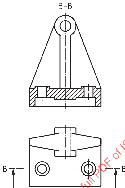
Figure D.2 — Section/cut in one plane
