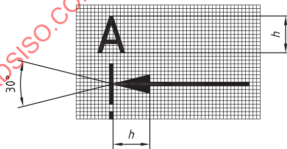
Figure A.3 — 30° cut and section arrow
