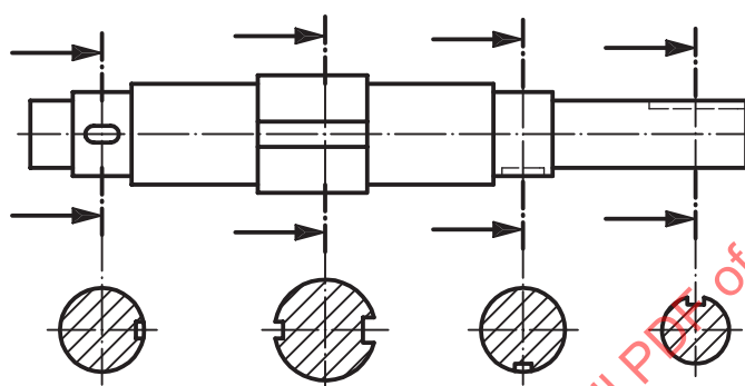
Figure D.9 — Successive sections/cuts — Example 2
