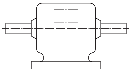
Figure C.7 — Indication of contours
