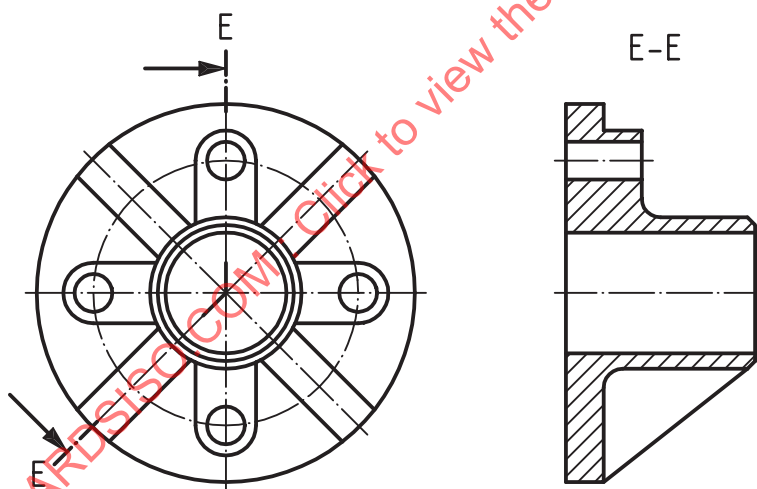
Figure D.5 — Section/cut in two intersecting planes
