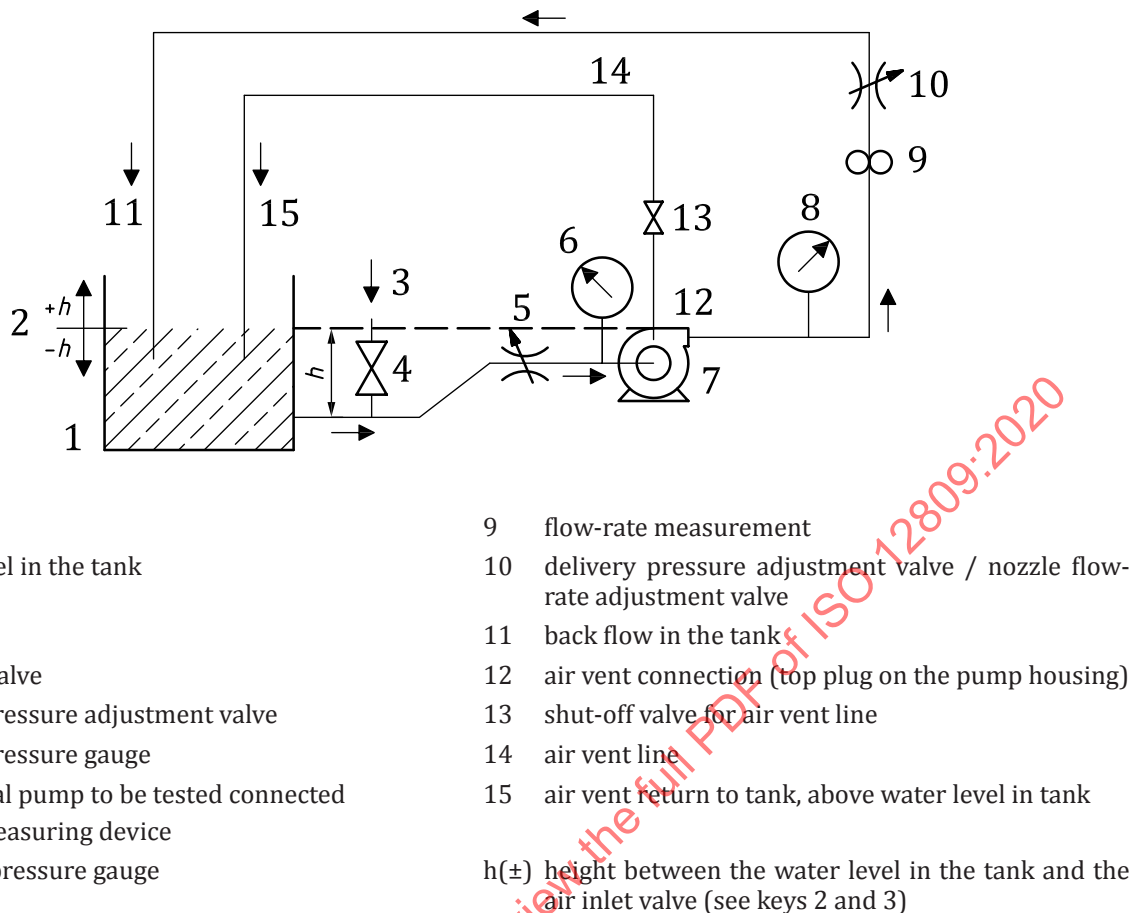
Figure 2 — Scheme of hydraulic circuit for non-self-priming centrifugal pump
