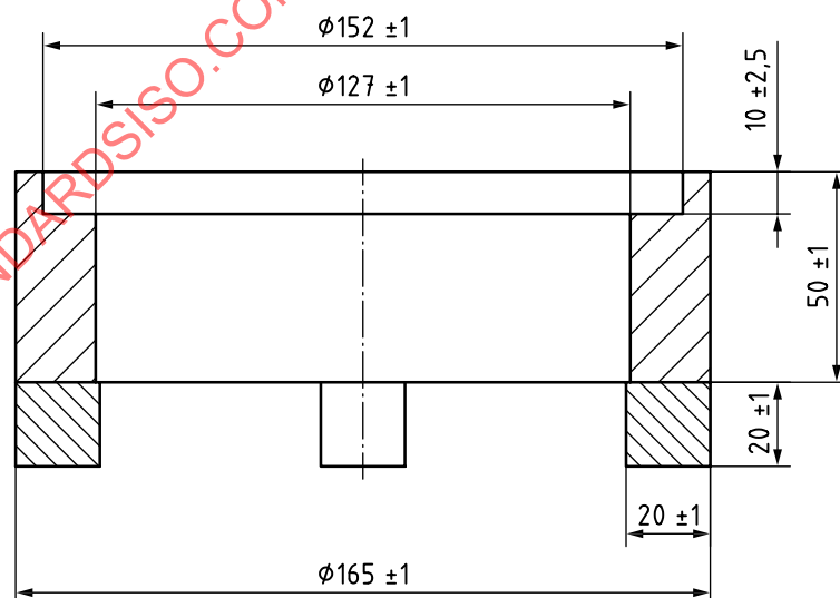
Figure A.4 — View of the substrate holder
