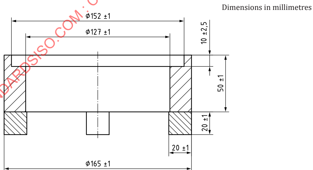
Figure A.4 — Cross-section of the substrate holder
