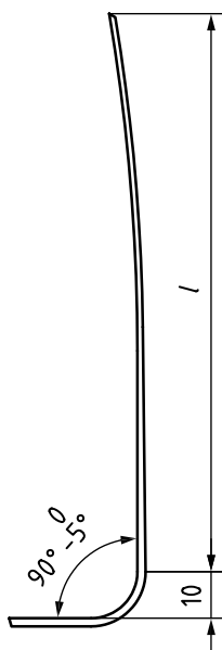
Figure 1 — Measurement of overall length of side for sides without a joint
