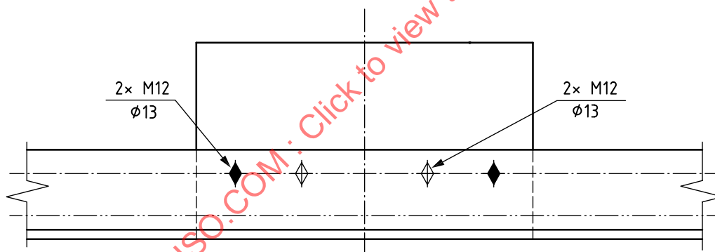
Figure 12 — Dimensioning of bolts
