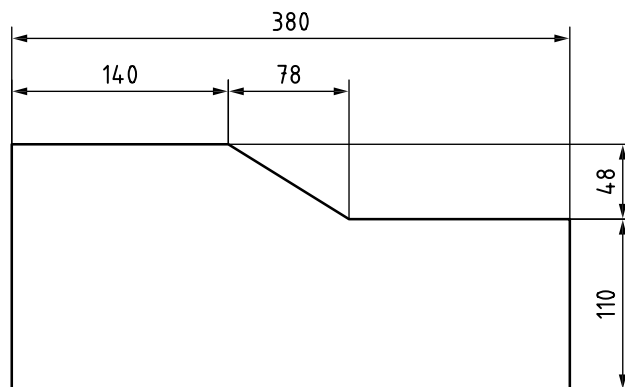
Figure 6 — Dimensioning of cutting plate
