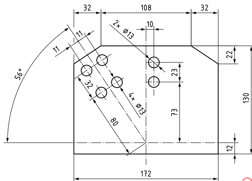
Figure 11 — Dimensioning of gusset plate
